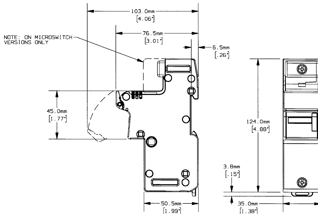
SIDE VIEW
